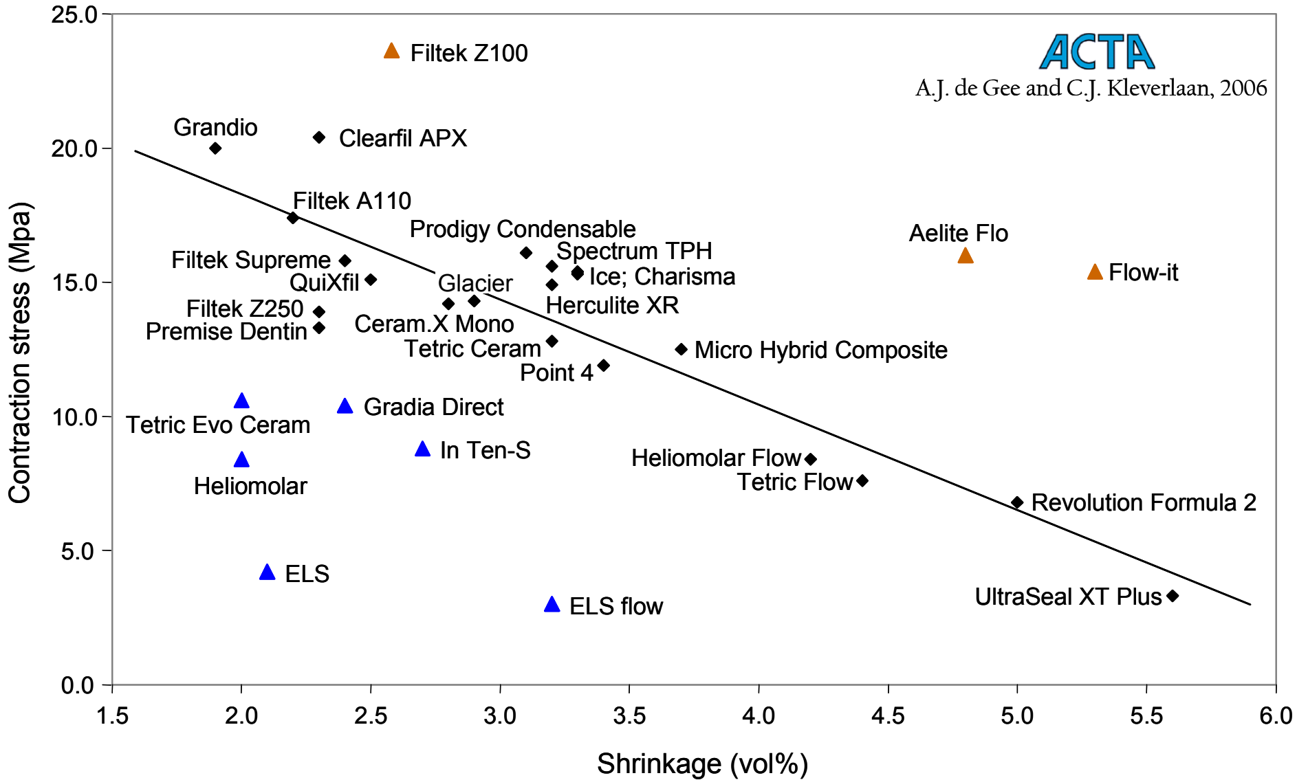
Regression plot of Volumetric Shrinkage and Contraction Stress (30 min values)
